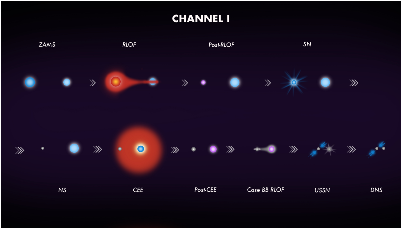
Figure 1: Graphical representation of the key stages in the evolution of a massive stellar binary leading to a double neutron star (Figure 1 of Vigna-Gómez et al. 2020 [3]).
