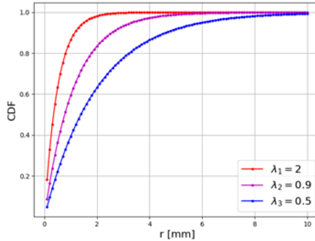
Figure 1: Cumulative Distribution Fonction
