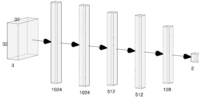
Figure 1: Architecture of ANN used for Image classification
